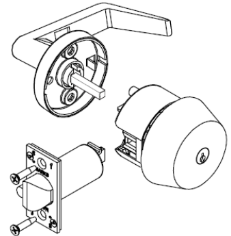
145KL Gatelatch Deadbolt w/ Lever
